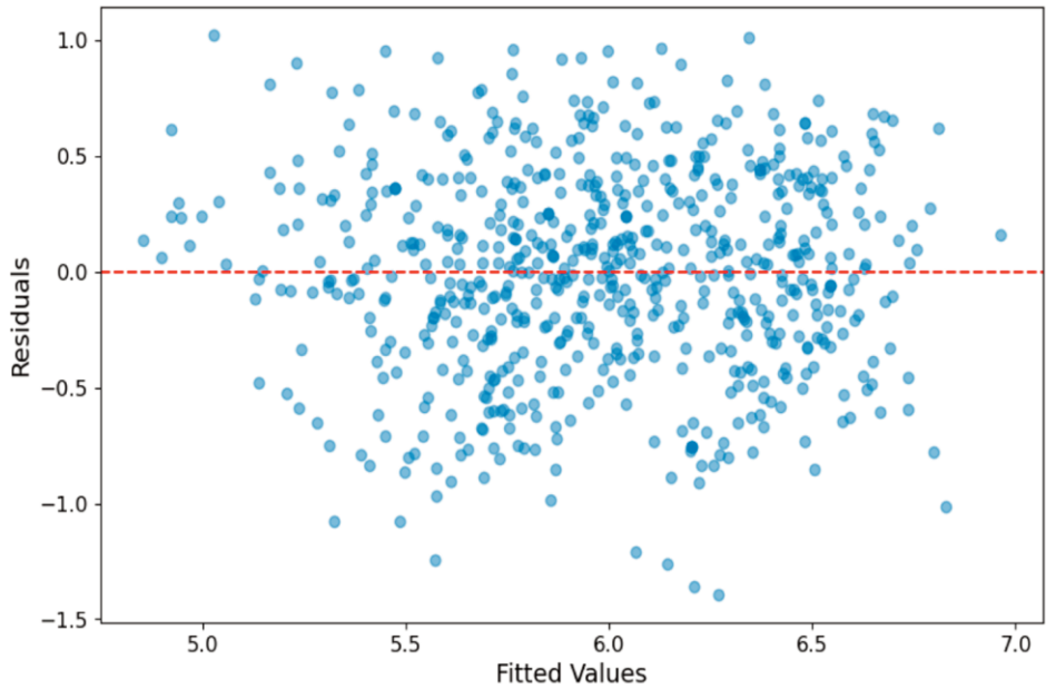
Figure A.1: Cost Model Residuals Compared to Fitted Values
